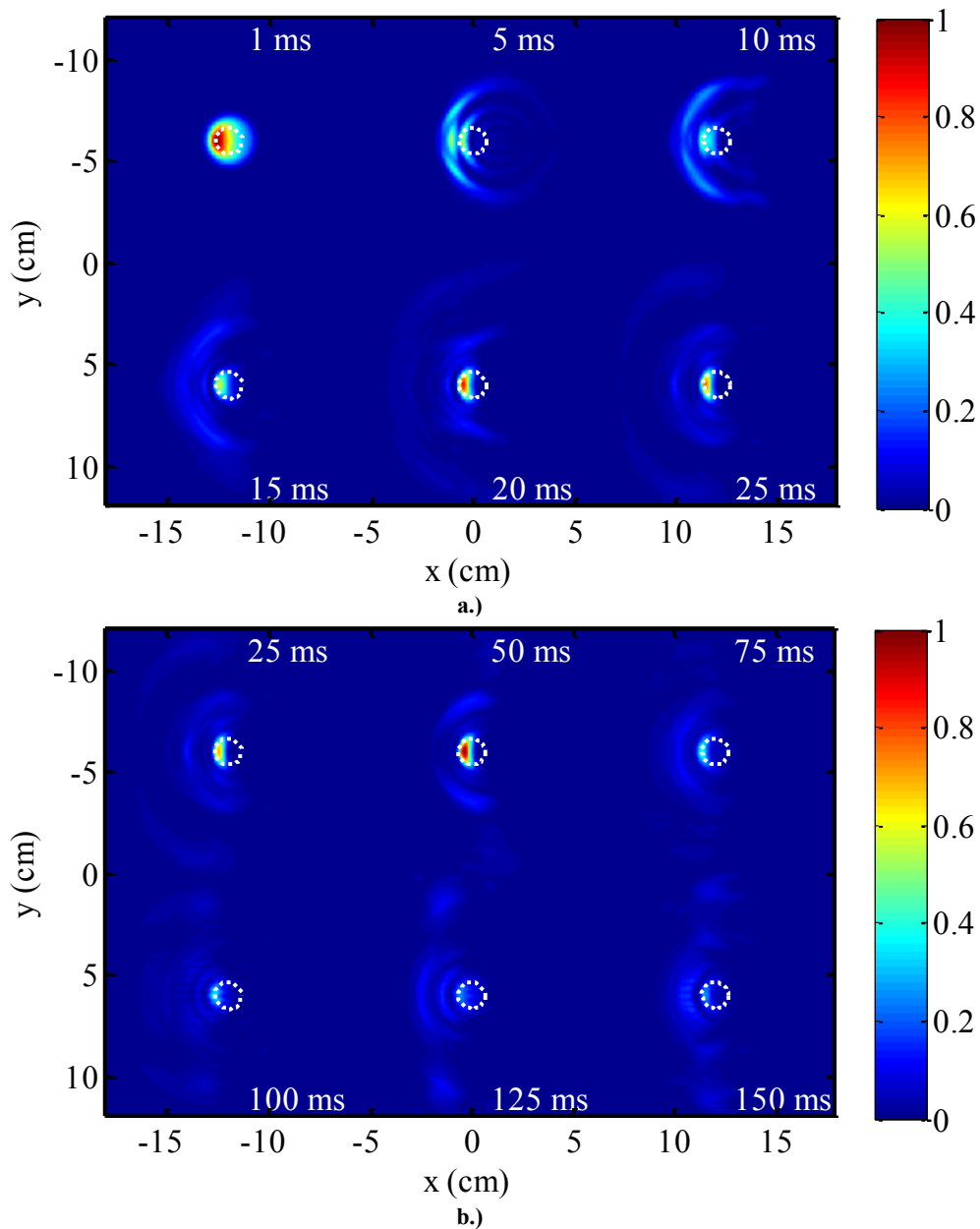
Figure 77. Normalized HEL beam irradiance with ab initio phase compensation of time-dependent thermal blooming for a distortion number, N_D=33.6 rad, 32 subapertures across the aperture, n_{\text{lod}}=32 , and eight waves of tilt per subaperture, n_{\text{lod}}=8 \lambda . In a.) the simulation runs from 1 ms to 25 ms and in b.) the simulation runs from 25 ms to 150 ms. The white circles represents the diffraction limited bucket diameter for the simulations, D_B=1.3 cm.
