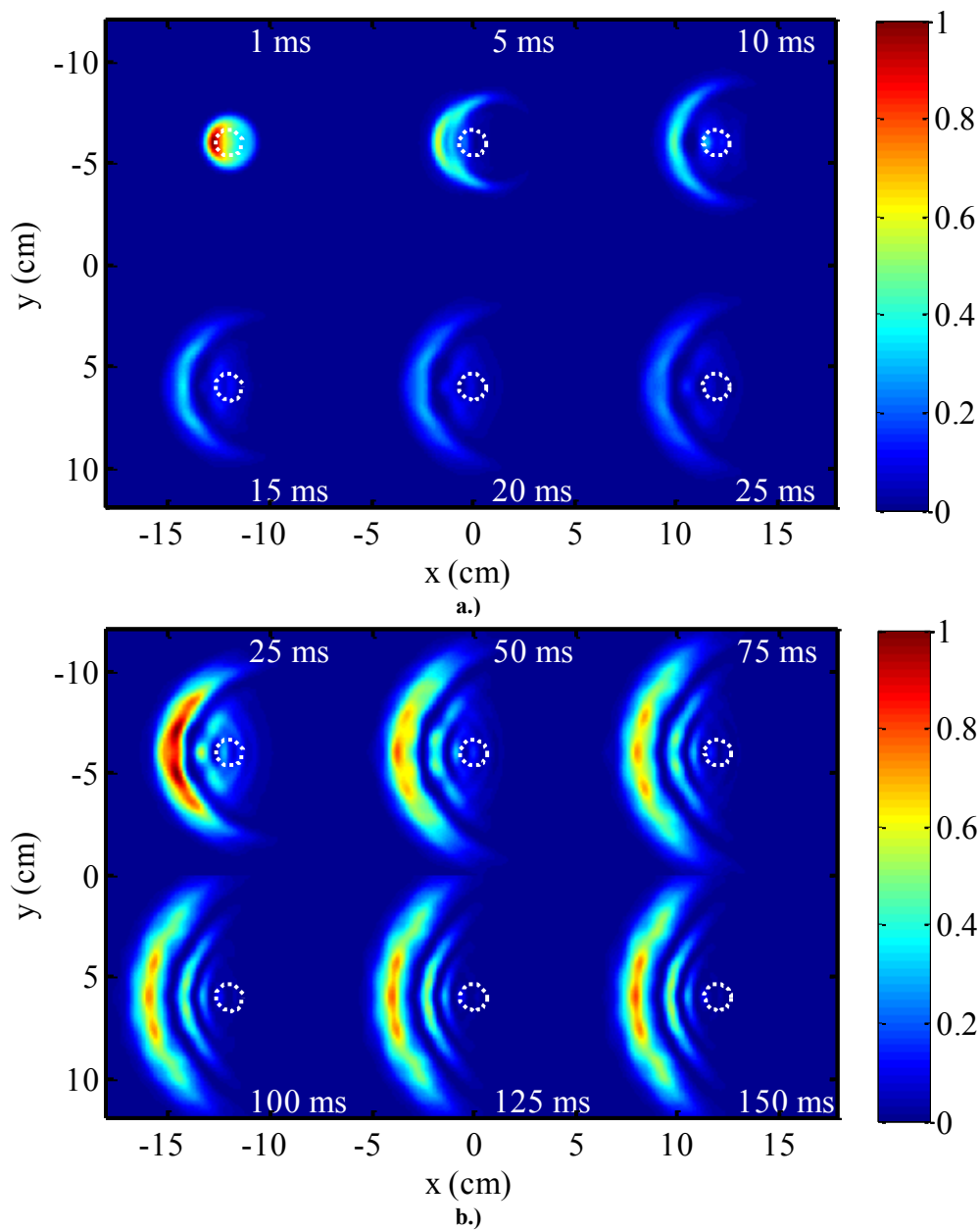
Figure 32. Normalized HEL beam irradiance for time-dependent thermal blooming and a distortion number well above the critical point, N_D=42.0 rad. In a.) the simulation runs from 1 ms to 25 ms and in b.) the simulation runs from 25 ms to 150 ms. The white circles represents the diffraction limited bucket diameter D_B=1.3 cm.
