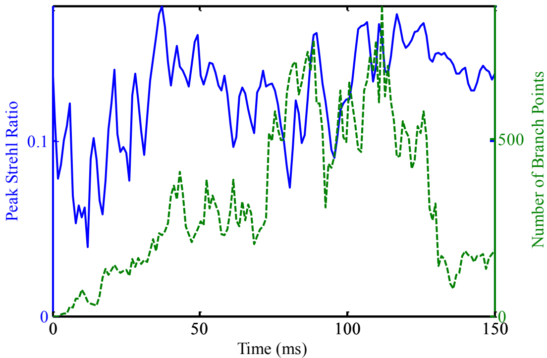
Figure 74. Comparison of peak Strehl ratio calculations in the target plane as a function of time with the number of branch points in the source plane as a function of time for a distortion number, N_D=38.8 rad, and a spherical-wave coherence diameter, r_{0,sw}=13.6 cm. The results show that the two measurements are anticorrelated for time-dependent turbulent thermal blooming and 25 independent realizations of optical turbulence.
