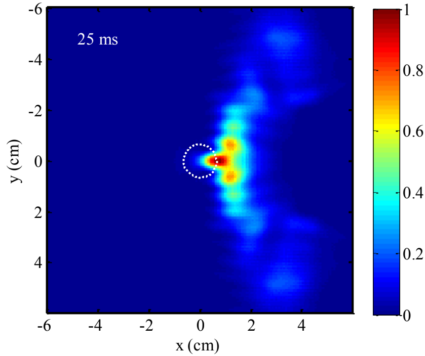
Figure 54. Simulation time stamp, t=25 ms, for normalized HEL beam irradiance with open-loop ab initio phase compensation of time-dependent thermal blooming and a distortion number, N_D=8.39 rad. The white circle represents the diffraction limited bucket diameter for the simulation, D_B=1.3 cm.
