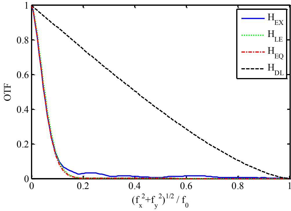
Figure 37. Optical turbulence validation study using the OTF. The experimental OTF H_{EX} is calculated from 25 independent realizations of a point source propagating through optical turbulence. The equivalent OTF is determined from the long-exposure and diffraction-limited OTF, H_{EQ}=H_{DL}H_{LE}
