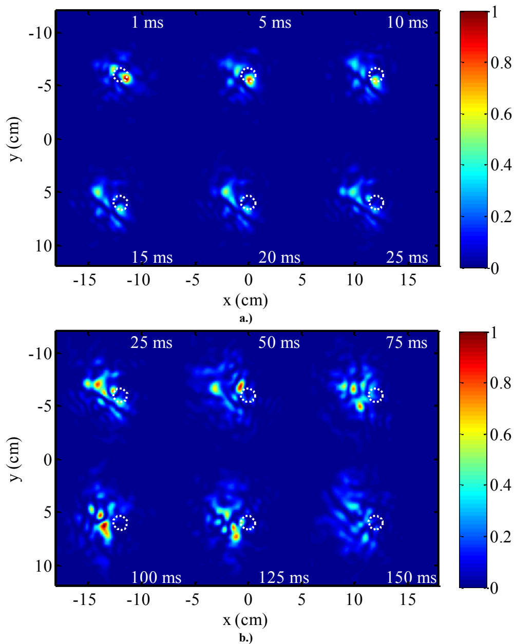
Figure 38. Normalized HEL beam irradiance with time-dependent thermal blooming and one realization of optical turbulence for a spherical-wave coherence diameter, r_{0,sw}=13.6 cm, and a distortion number, N_D=16.7 rad. In a.) the simulation runs from 1 ms to 25 ms and in b.) the simulation runs from 25 ms to 150 ms. The white circles represents the diffraction limited bucket diameter for the simulations, D_B=1.3 cm.
