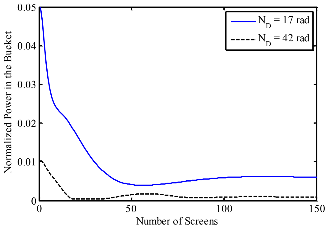
Figure 27. Thermal blooming phase screen convergence study using a.) peak Strehl ratio versus number of screens and b.) normalized power in the bucket versus number of screens.
