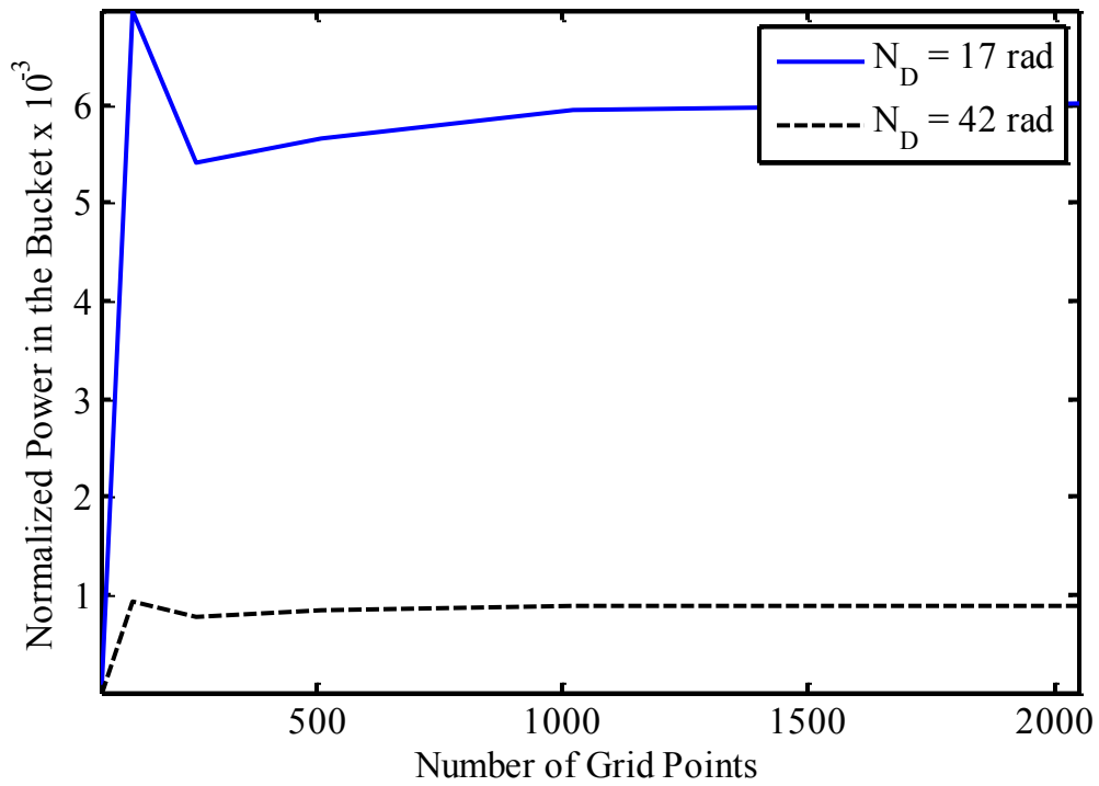
Figure 28. Number of grid points convergence study using a.) peak Strehl ratio versus number of grid points and b.) normalized power in the bucket versus number of grid points.
