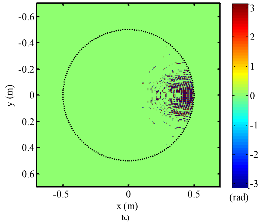
Figure 65. The highest number of branch points present in the source plane with an initial phase compensation of time-dependent thermal blooming for a distortion number, N_D=42.0 rad. In a.) the point-source beacon wrapped phase for the t=87 ms time stamp is given and in b.) the associated placement of the branch points is given.
