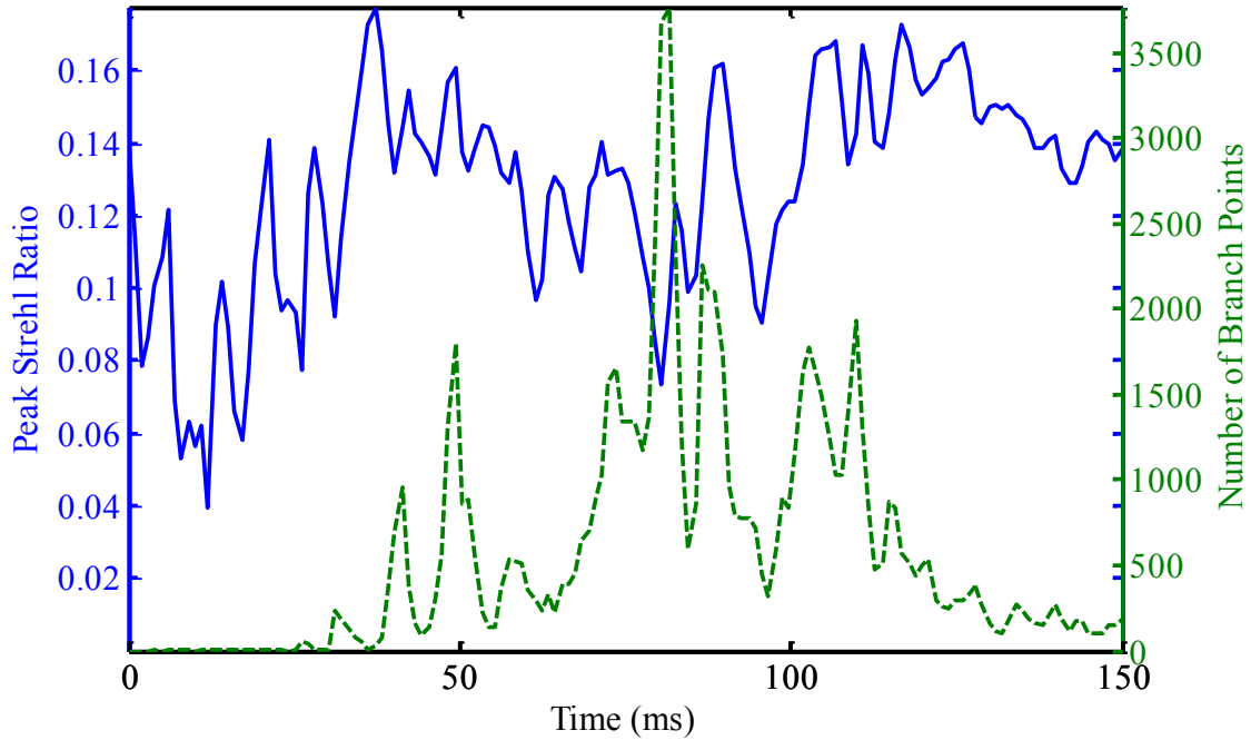
Figure 66. Comparison of peak Strehl ratio calculations in the target plane as a function of time with the number of branch points in the source plane as a function of time for a distortion number, N_D=42.0 rad, 16 subapertures across the aperture, n_{\text{tod}}=32 , and ten waves of tilt per subaperture, n_{\text{tod}}=10 \lambda . The results show that the two measurements are correlated for time-dependent thermal blooming.
