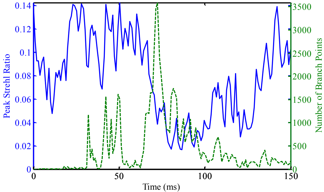
Figure 70. Comparison of peak Strehl ratio calculations in the target plane as a function of time with the number of branch points in the source plane as a function of time for a distortion number, N_D=42.0 rad, 32 subapertures across the aperture, n_{\text{lod}}=32 , and ten waves of tilt per subaperture, n_{\text{lod}}=10 \lambda . The results show that the two measurements are anticorrelated for time-dependent thermal blooming.
