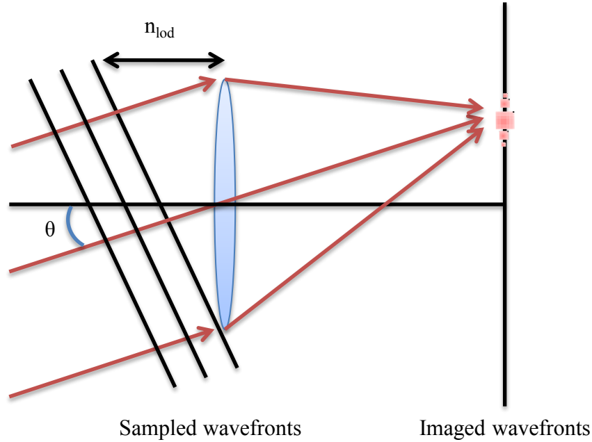
Figure 13. Description of the FOV \theta of a Shack-Hartmann WFS subaperture. The number of waves of tilt n_{\text{tod}} is related to the FOV \theta using simple geometric relationships.
