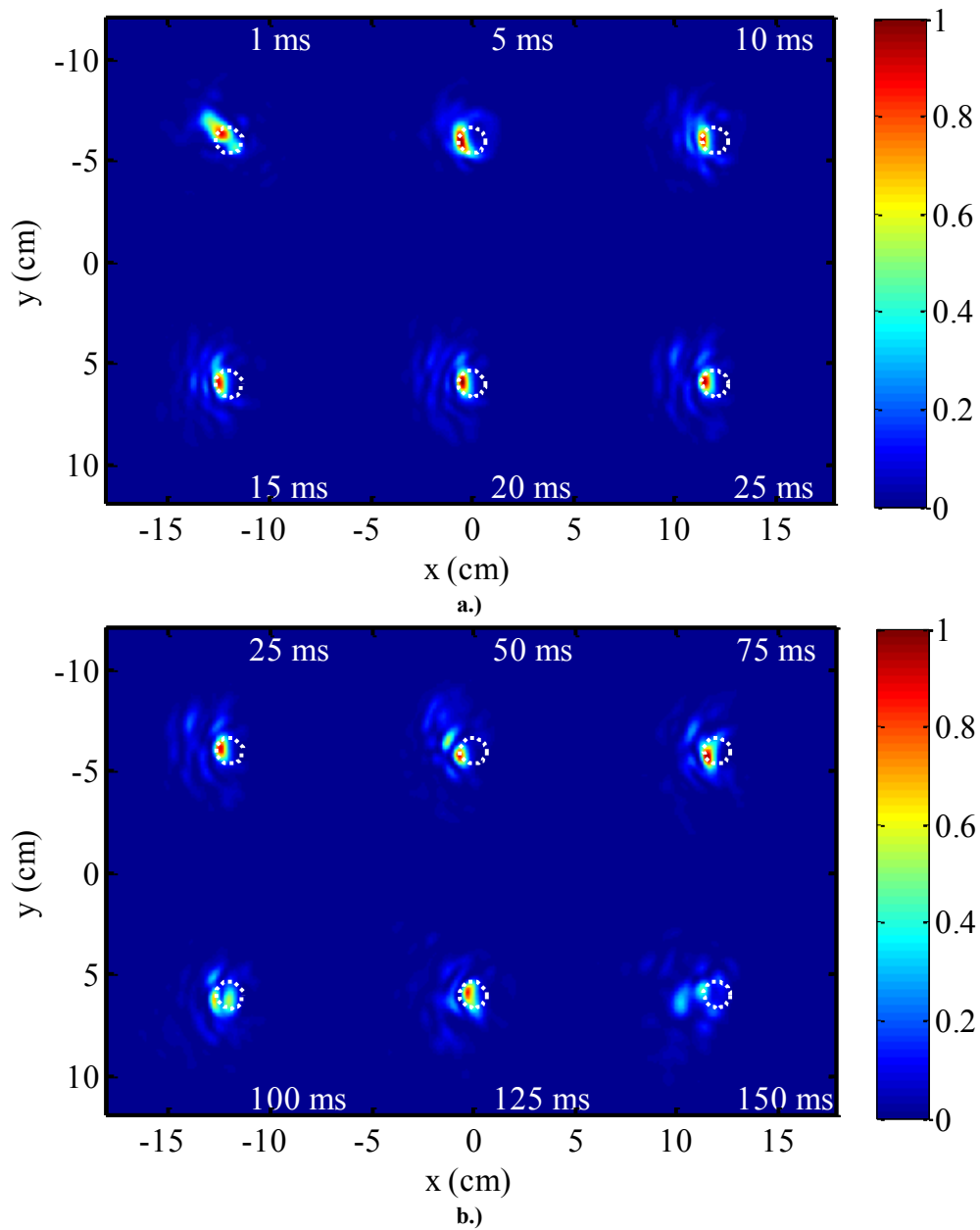
Figure 57. Normalized HEL beam irradiance with ab initio phase compensation of time-dependent turbulent thermal blooming and one realization of optical turbulence for a distortion number, N_D=15.5 rad, a wind velocity standard deviation, \sigma_v=1.8 m/s, and a spherical coherence diameter, r_{0,sv}=13.6 cm. In a.) the simulation runs from 1 ms to 25 ms and in b.) the simulation runs from 25 ms to 150 ms. The white circles represents the diffraction limited bucket diameter for the simulations, D_B=1.3 cm.
